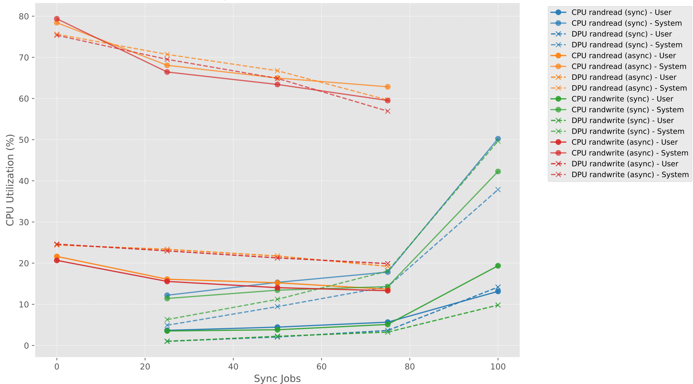
CPU Utilization vs Sync Jobs (mixed) - RAND (CPU vs DPU)
